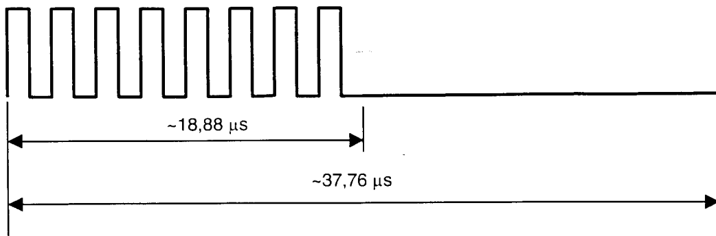
Figure 10 — Logic 0
