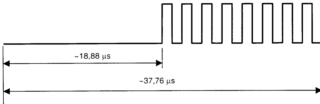
Figure 11 — Logic 1
