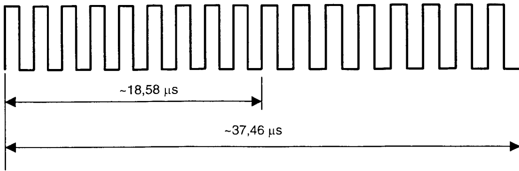
Figure 13 — Logic 1
