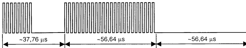
Figure 16 — End of frame when using one subcarrier
